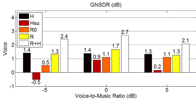
Fig. 2. Separation performance via the GNSDR in dB, for the voice component, at voice-to-music ratios of -5 , 0 , and 5 dB, from left to right, using only a high-pass filtering ( H , black), Hsu’s system ( Hsu , dark color), the initial REPET with binary masking ( R0 , medium color), REPET (with soft masking) ( R , light color), and REPET plus high-pass filtering ( R + H , white). Higher values are better.
